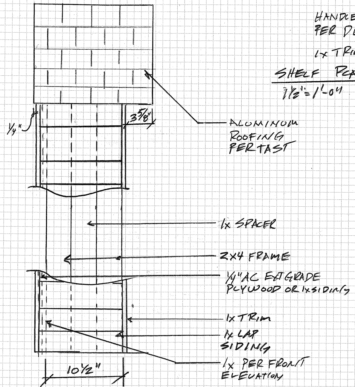
SIDE ELEVATION 1\frac{1}{2}'' = 1'-0''
