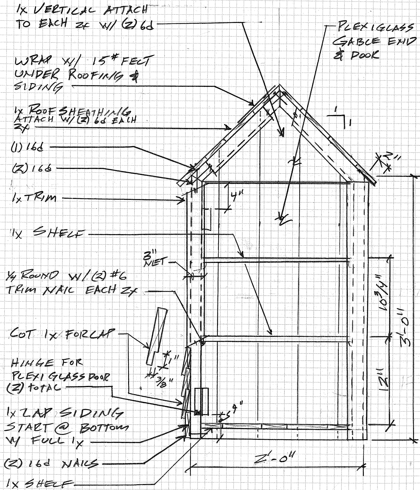
FRONT ELEVATION 1\frac{1}{2}'' = 1'-0''
