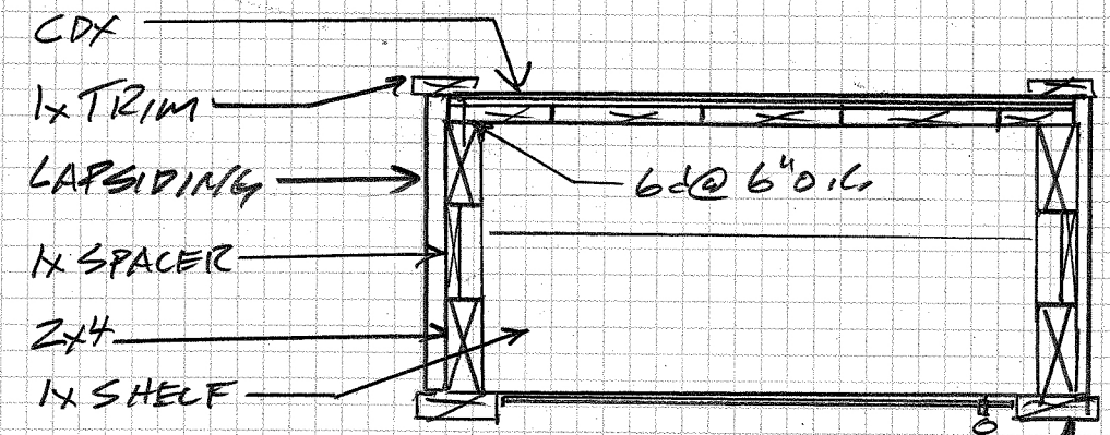
SHELF PLAN VIEW 1\frac{1}{2}'' = 1'-0''
