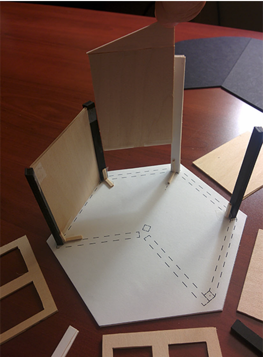
Install posts, screw to base with metal angle
