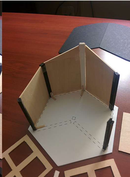
Slide panels in between the posts, caulk around edges
