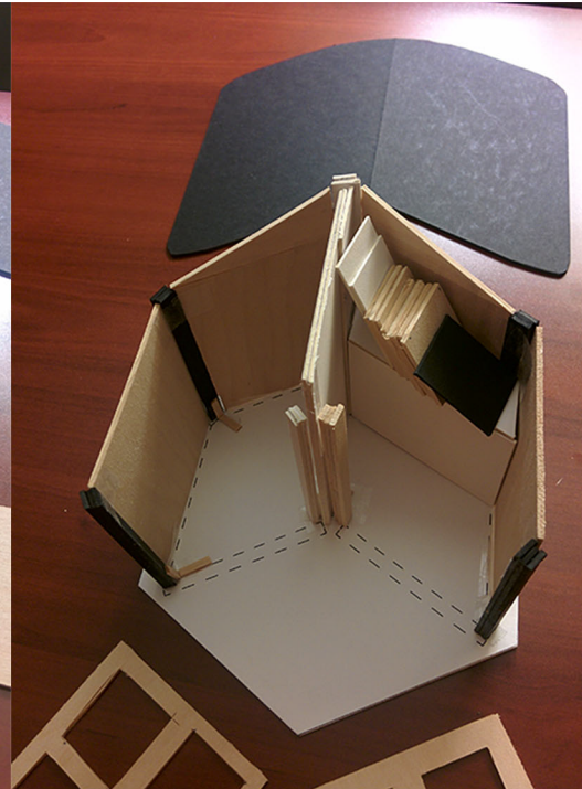
Install interior panel and shelf, screwing to base and posts
